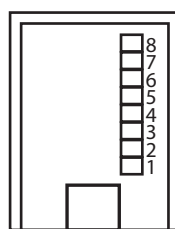
Gniazdo RJ45
