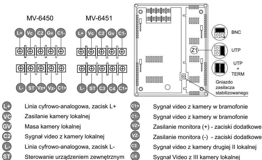
Rys. 7.5 Zaciski wideomonitora
