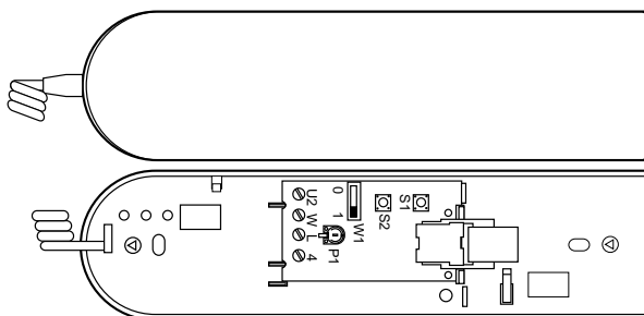
Rys. 3.3 Unifon LM-16.
